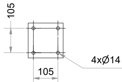
Transmitter Holes Detail ( 1 : 10 )
