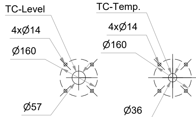
Transmitter Holes Detail ( 1 : 10 )
