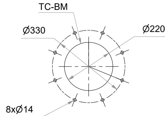
Biomass Holes Detail ( 1 : 10 )
