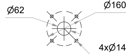
Anti Foam Holes Detail ( 1 : 10 )
